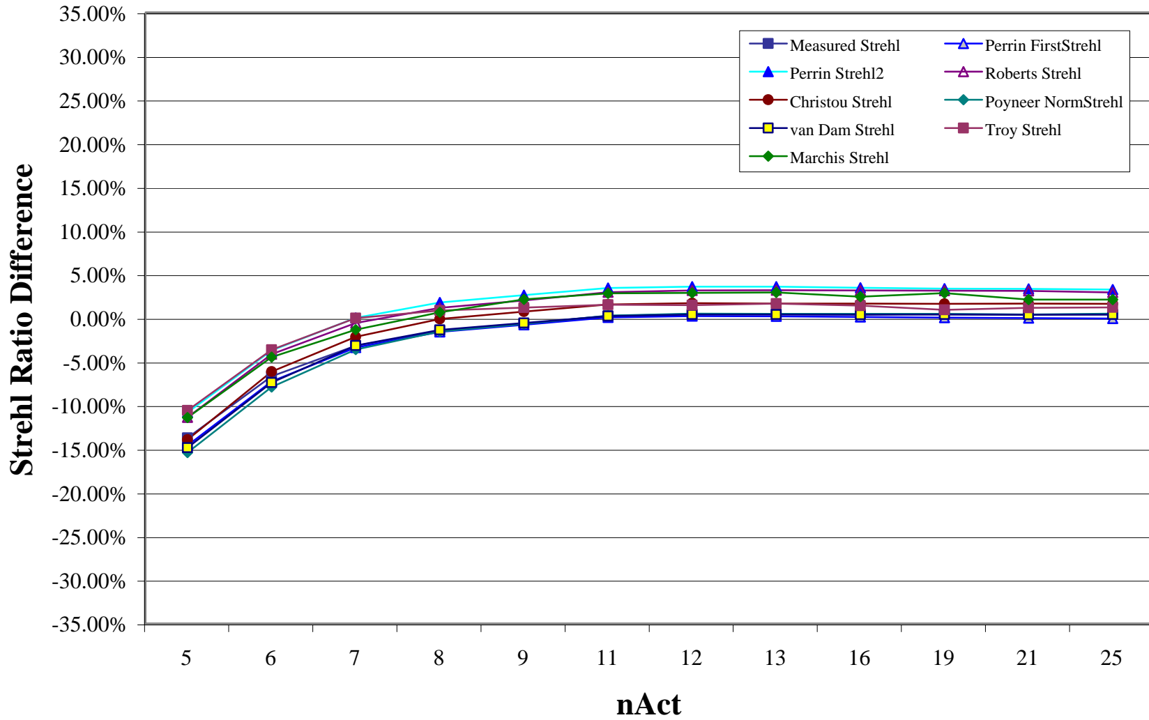
StrehlCampaign Results: 2 x Nyquist Sampling ( \lambda/4D )
